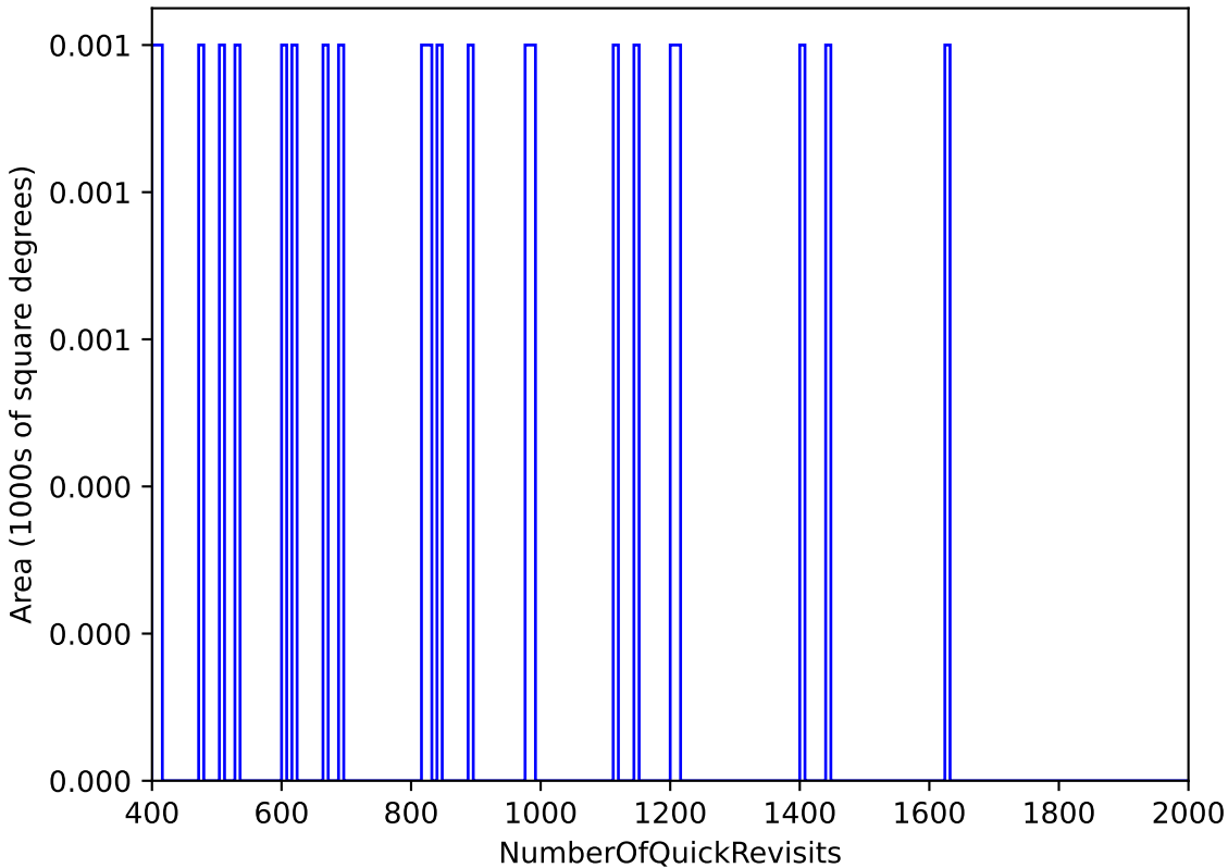
too_elab_heavy_r128_d2_ugrizy_v3.4_10yrs : NumberOfQuickRevisits
