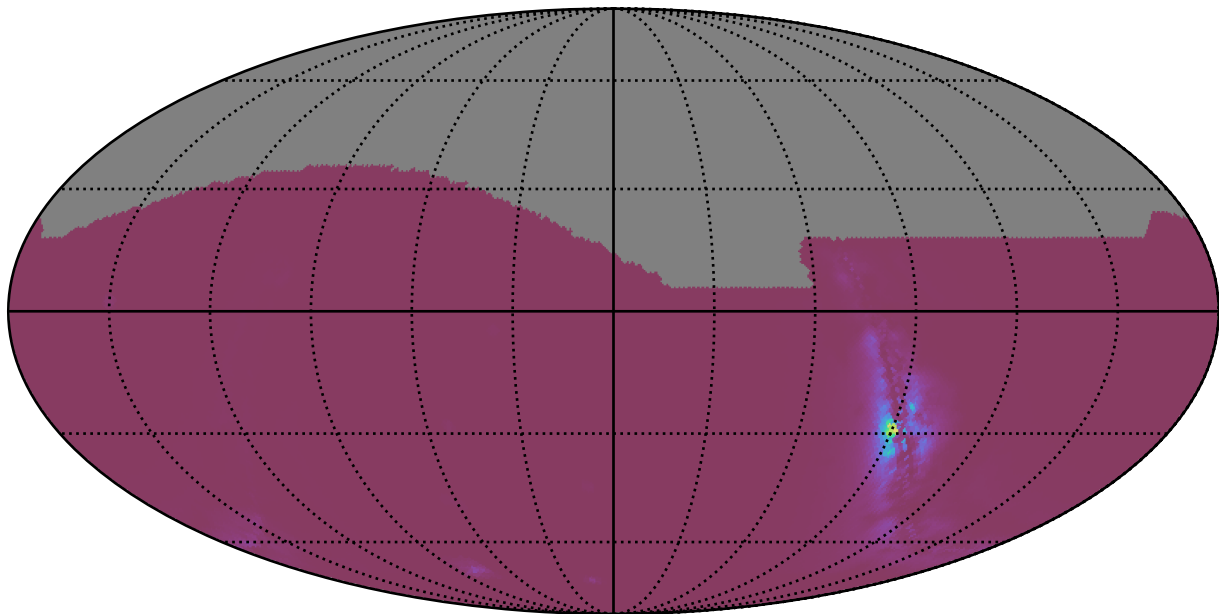
too_elab_heavy_r128_d2_ugrizy_v3.4_10yrs : NlcPoints
