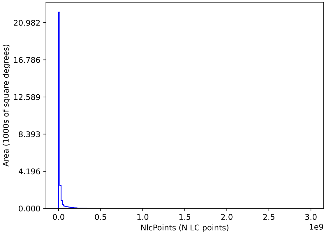
too_elab_heavy_r128_d2_ugrizy_v3.4_10yrs : NlcPoints
