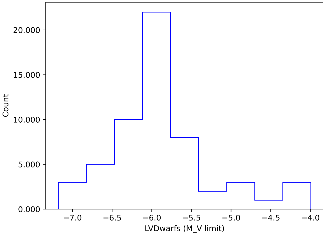
too_elab_heavy_r128_d2_ugrizy_v3.4_10yrs gi: LVDwarfs
