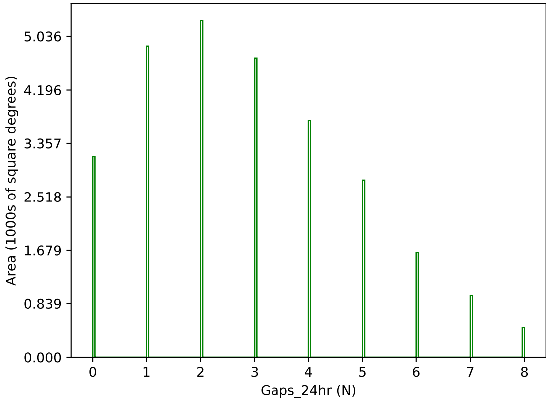
too_elab_heavy_r128_d2_ugrizy_v3.4_10yrs g band: Gaps_24hr
