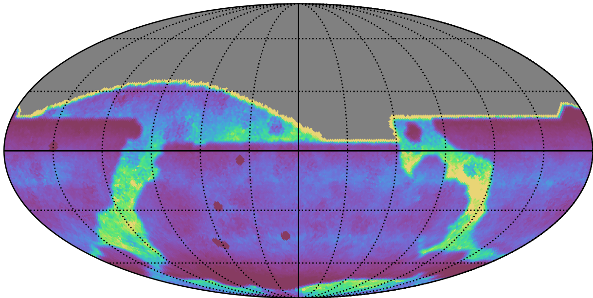
too_elab_heavy_r128_d2_ugrizy_v3.4_10yrs : DCRprecision
