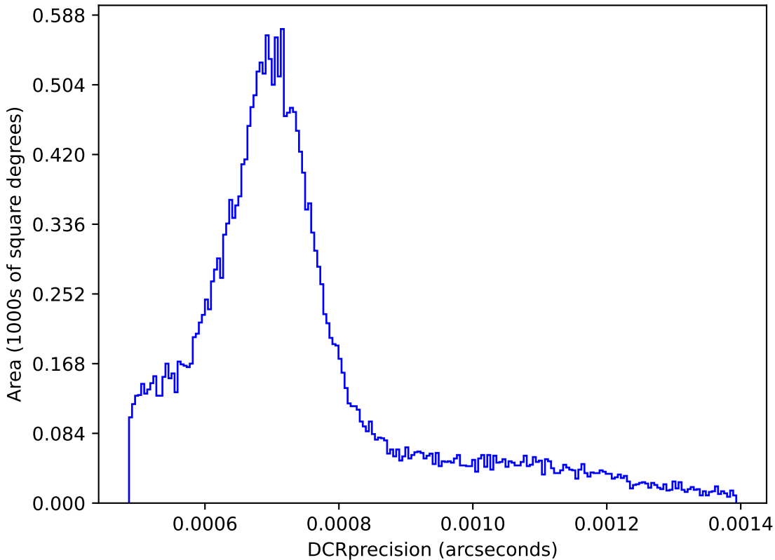
too_elab_heavy_r128_d2_ugrizy_v3.4_10yrs : DCRprecision
