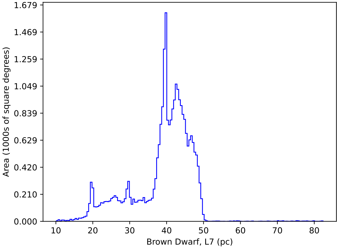
too_elab_heavy_r128_d2_ugrizy_v3.4_10yrs : Brown Dwarf, L7
