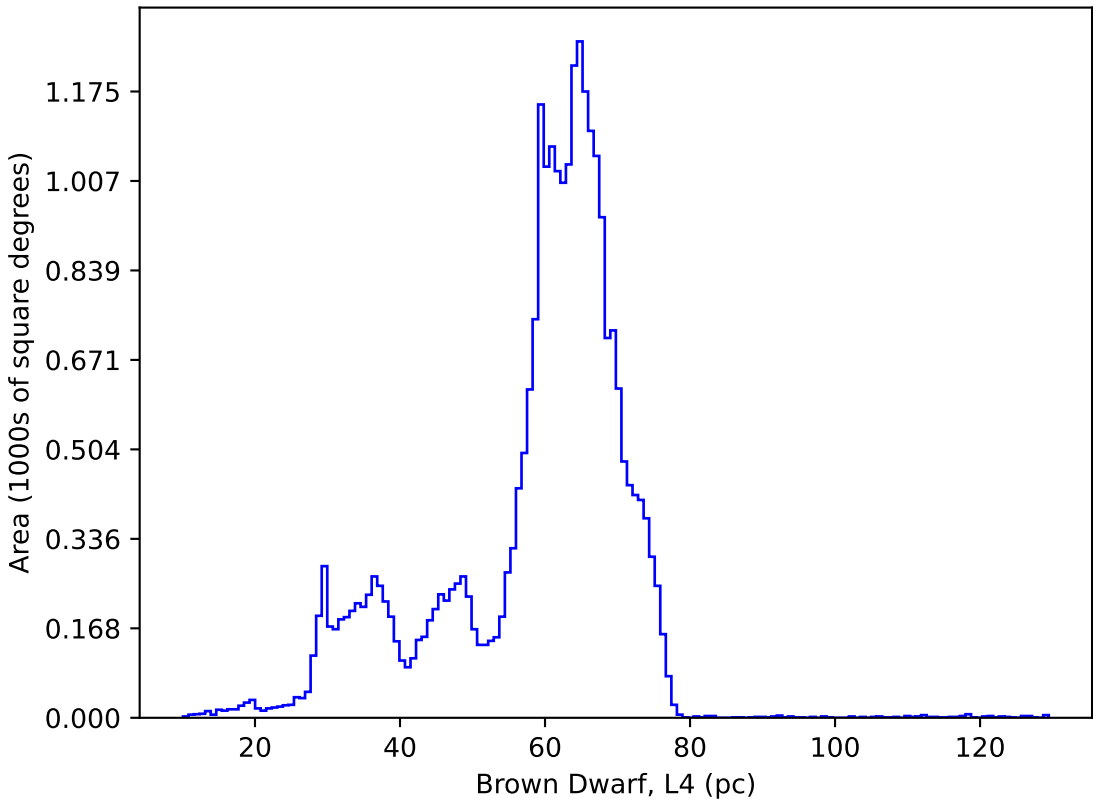
too_elab_heavy_r128_d2_ugrizy_v3.4_10yrs : Brown Dwarf, L4
