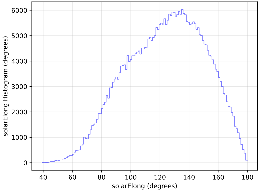
too_elab_heavy_r128_d2_ugrizy_v3.4_10yrs WFD y band: solarElong Histogram
