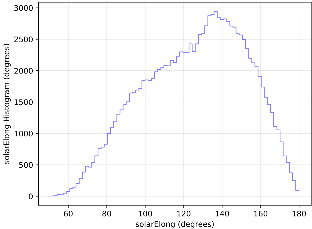
too_elab_heavy_r128_d2_ugrizy_v3.4_10yrs WFD u band: solarElong Histogram
