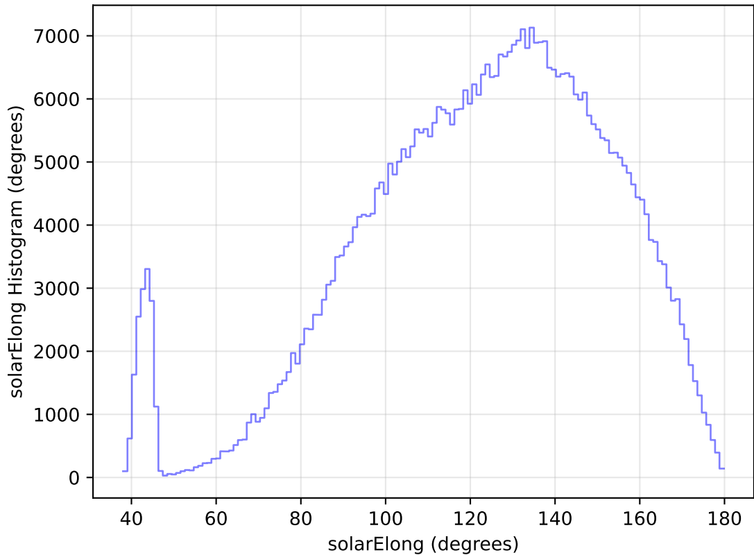
too_elab_heavy_r128_d2_ugrizy_v3.4_10yrs WFD r band: solarElong Histogram
