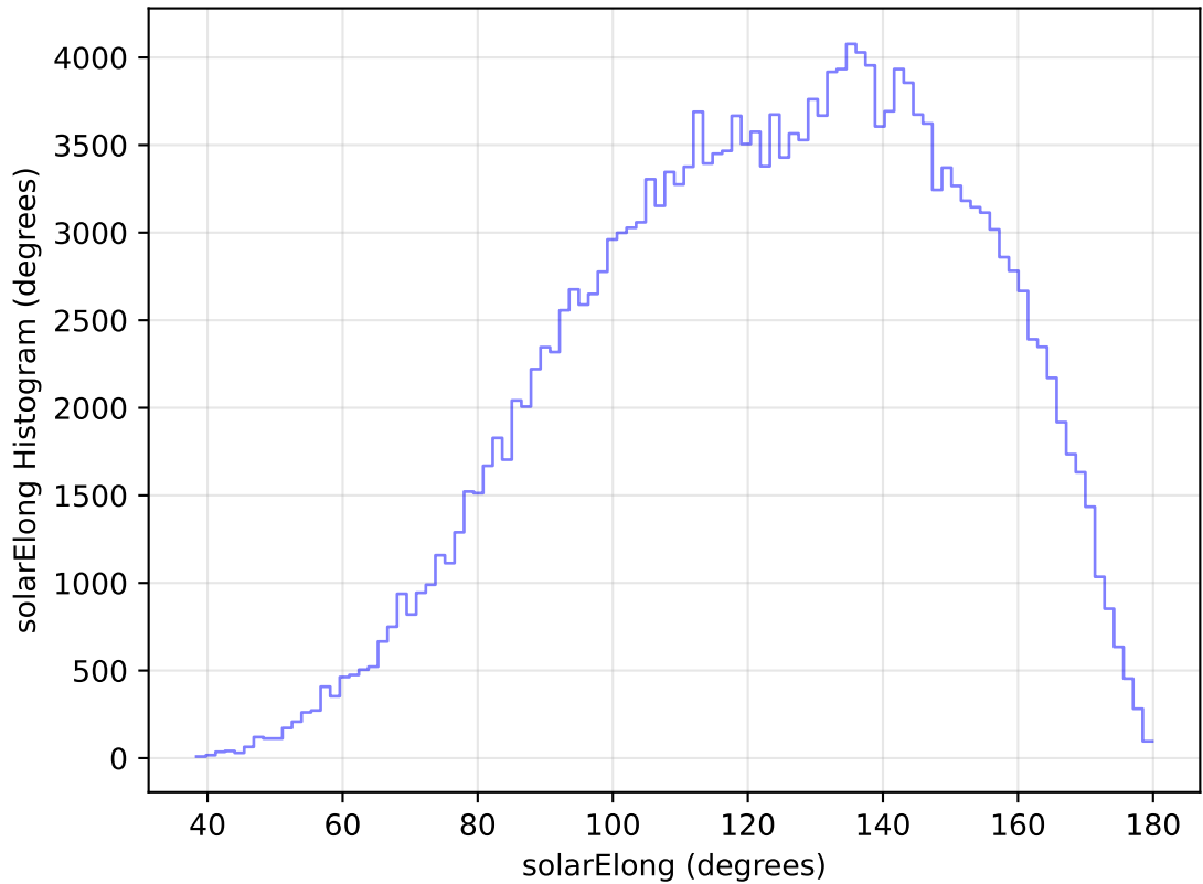
too_elab_heavy_r128_d2_ugrizy_v3.4_10yrs WFD g band: solarElong Histogram
