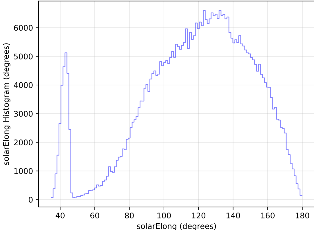
too_elab_heavy_r128_d2_ugrizy_v3.4_10yrs All sky z band: solarElong Histogram
