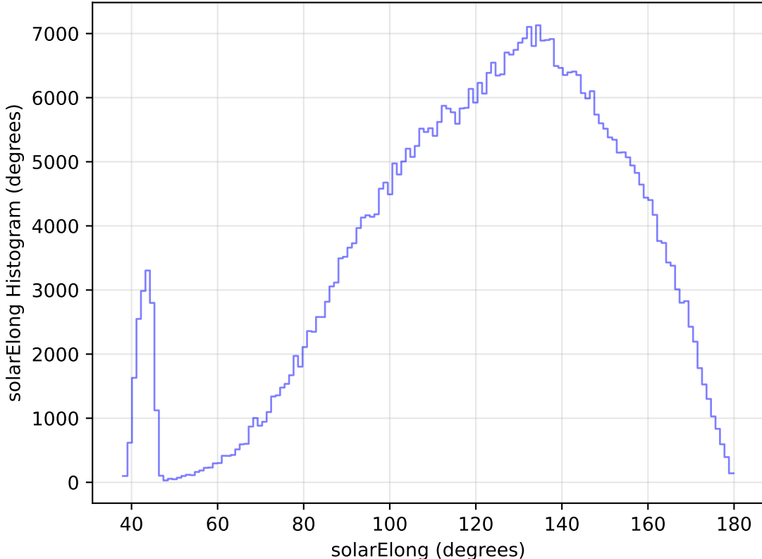
too_elab_heavy_r128_d2_ugrizy_v3.4_10yrs All sky r band: solarElong Histogram
