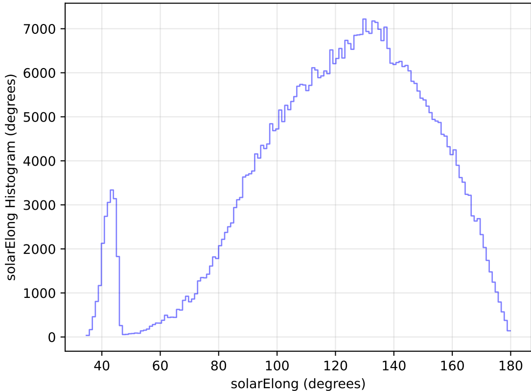
too_elab_heavy_r128_d2_ugrizy_v3.4_10yrs All sky i band: solarElong Histogram
