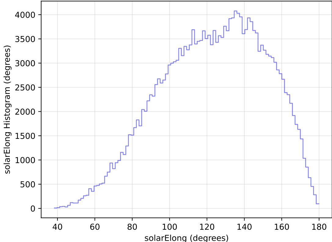
too_elab_heavy_r128_d2_ugrizy_v3.4_10yrs All sky g band: solarElong Histogram
