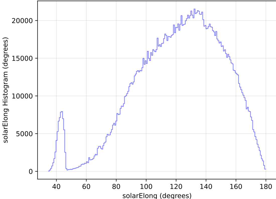
too_elab_heavy_r128_d2_ugrizy_v3.4_10yrs All sky all bands: solarElong Histogram
