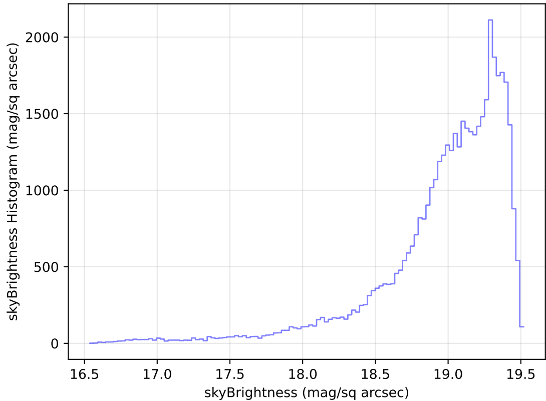
too_elab_heavy_r128_d2_ugrizy_v3.4_10yrs Yr 1 z band: skyBrightness Histogram
