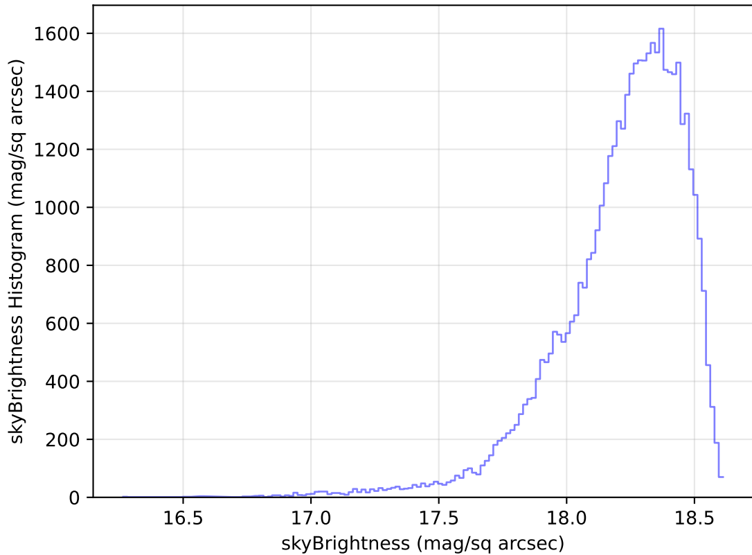
too_elab_heavy_r128_d2_ugrizy_v3.4_10yrs Yr 1 y band: skyBrightness Histogram
