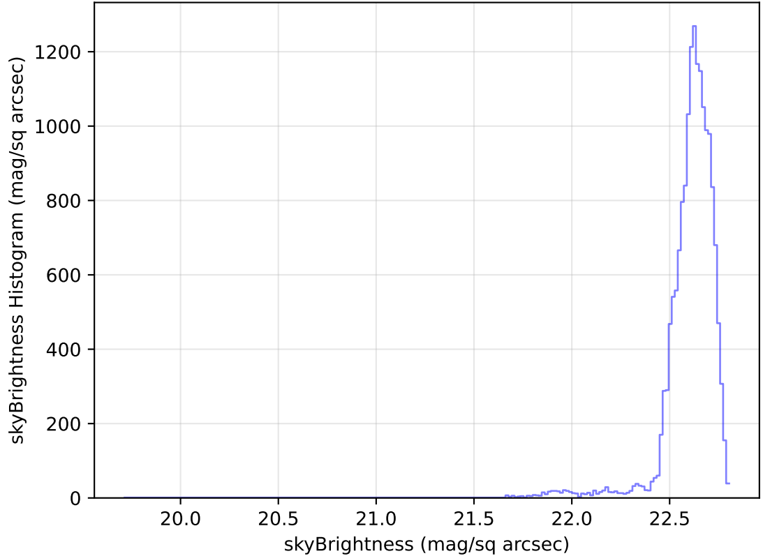
too_elab_heavy_r128_d2_ugrizy_v3.4_10yrs Yr 1 u band: skyBrightness Histogram
