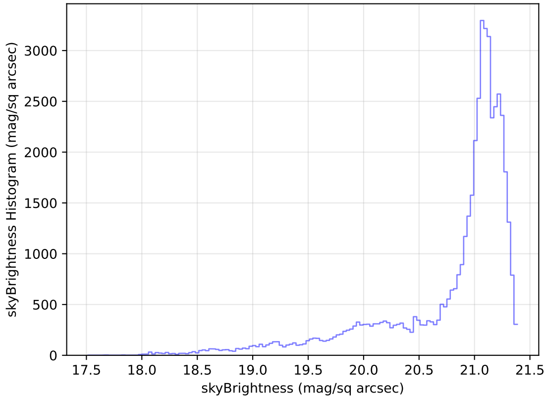
too_elab_heavy_r128_d2_ugrizy_v3.4_10yrs Yr 1 r band: skyBrightness Histogram
