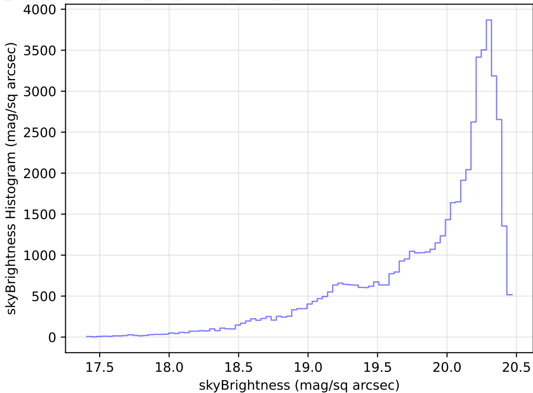
too_elab_heavy_r128_d2_ugrizy_v3.4_10yrs Yr 1 i band: skyBrightness Histogram
