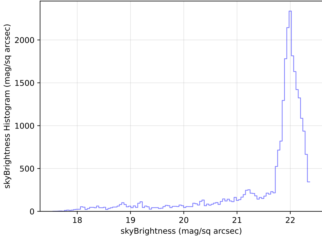
too_elab_heavy_r128_d2_ugrizy_v3.4_10yrs Yr 1 g band: skyBrightness Histogram
