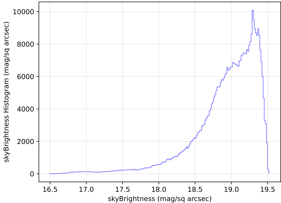
too_elab_heavy_r128_d2_ugrizy_v3.4_10yrs WFD z band: skyBrightness Histogram
