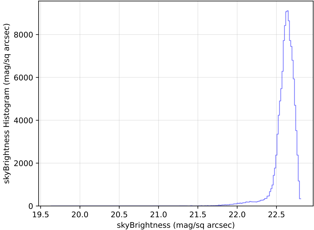
too_elab_heavy_r128_d2_ugrizy_v3.4_10yrs WFD u band: skyBrightness Histogram
