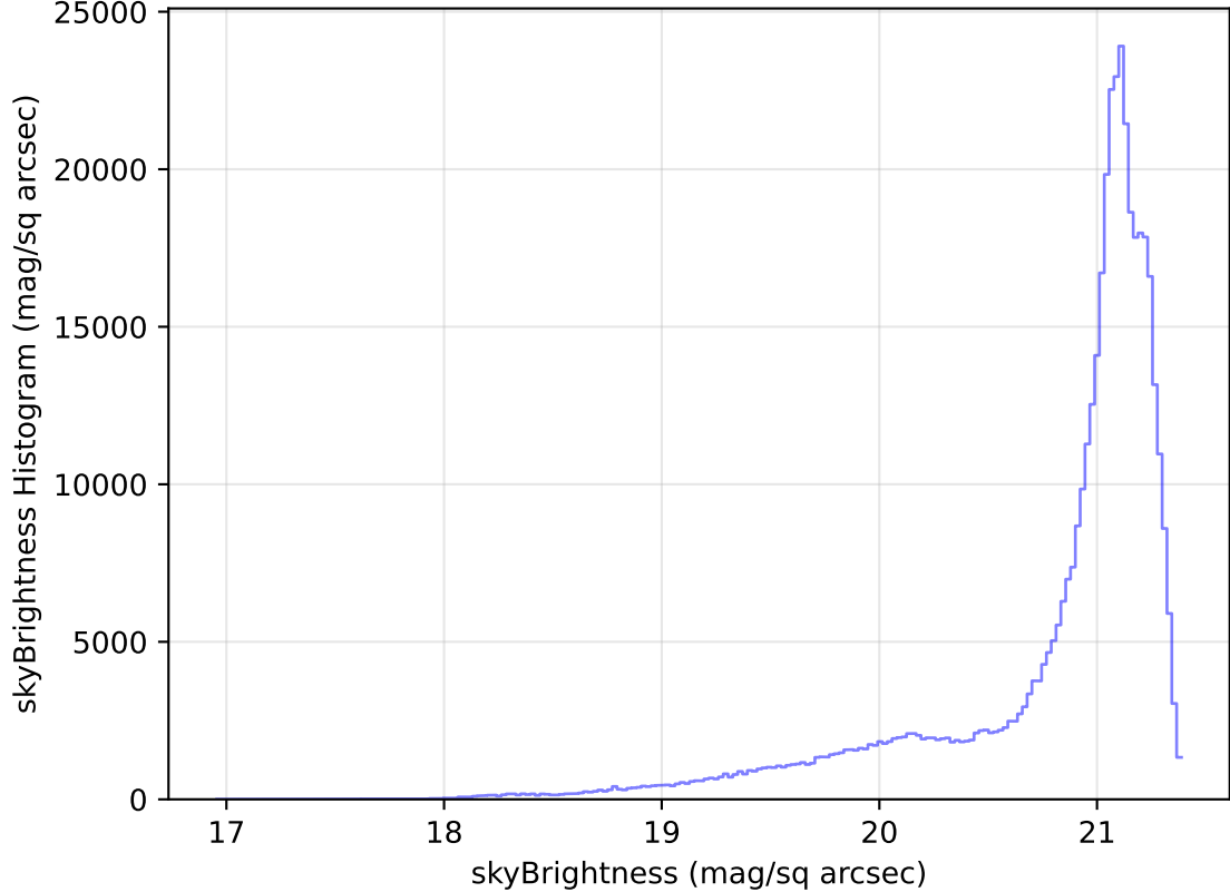
too_elab_heavy_r128_d2_ugrizy_v3.4_10yrs WFD r band: skyBrightness Histogram
