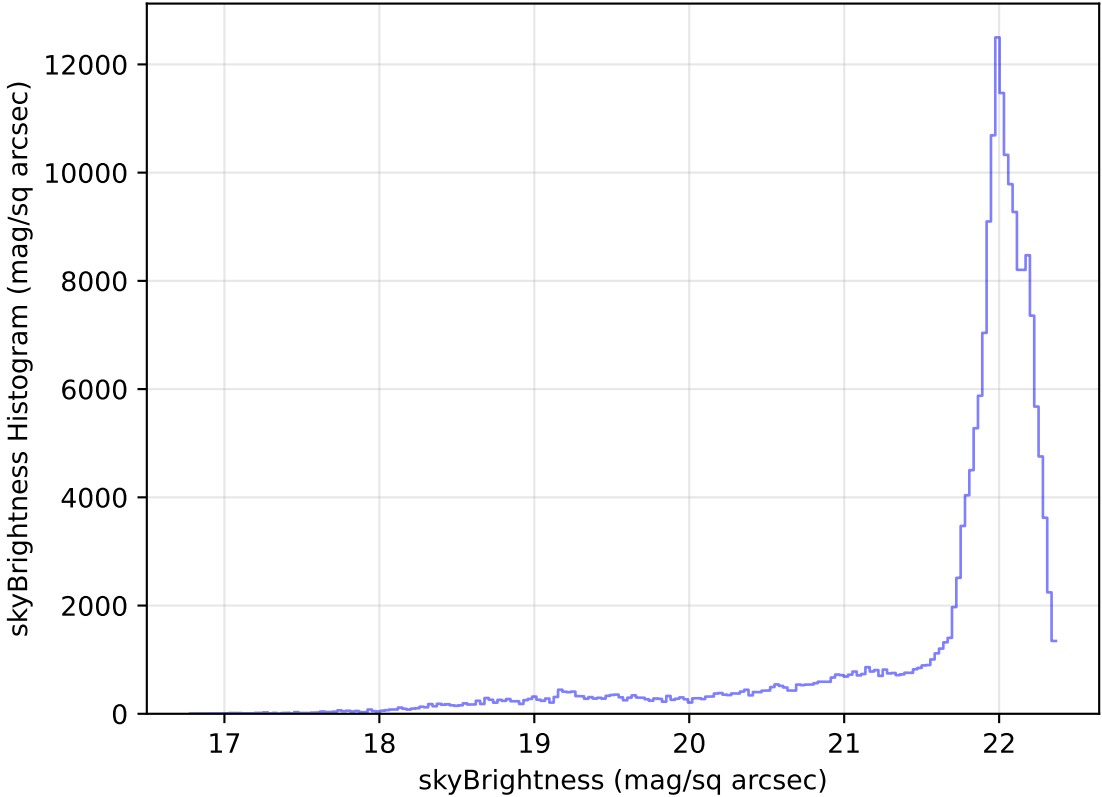
too_elab_heavy_r128_d2_ugrizy_v3.4_10yrs WFD g band: skyBrightness Histogram
