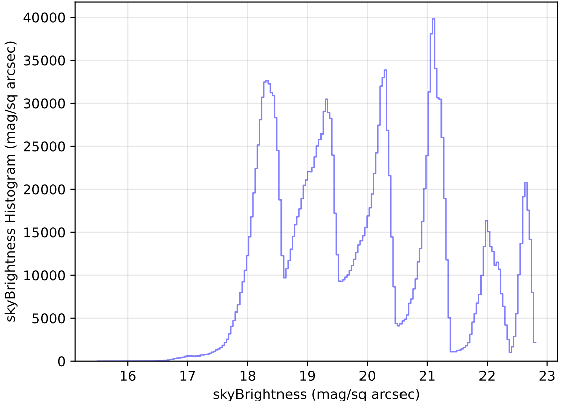
too_elab_heavy_r128_d2_ugrizy_v3.4_10yrs WFD all bands: skyBrightness Histogram
