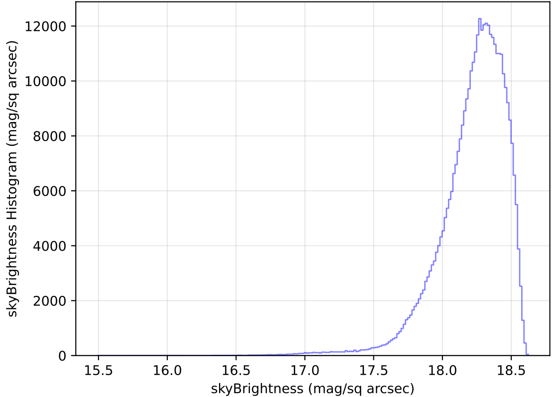
too_elab_heavy_r128_d2_ugrizy_v3.4_10yrs All sky y band: skyBrightness Histogram
