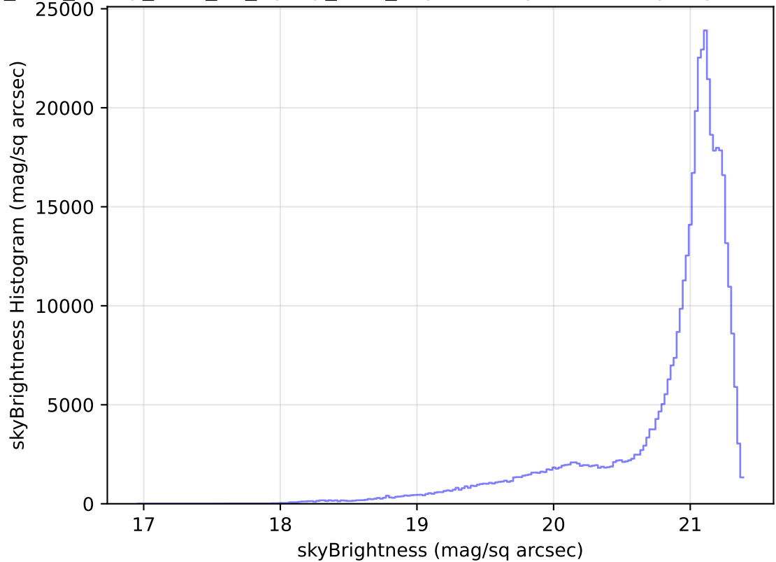
too_elab_heavy_r128_d2_ugrizy_v3.4_10yrs All sky r band: skyBrightness Histogram
