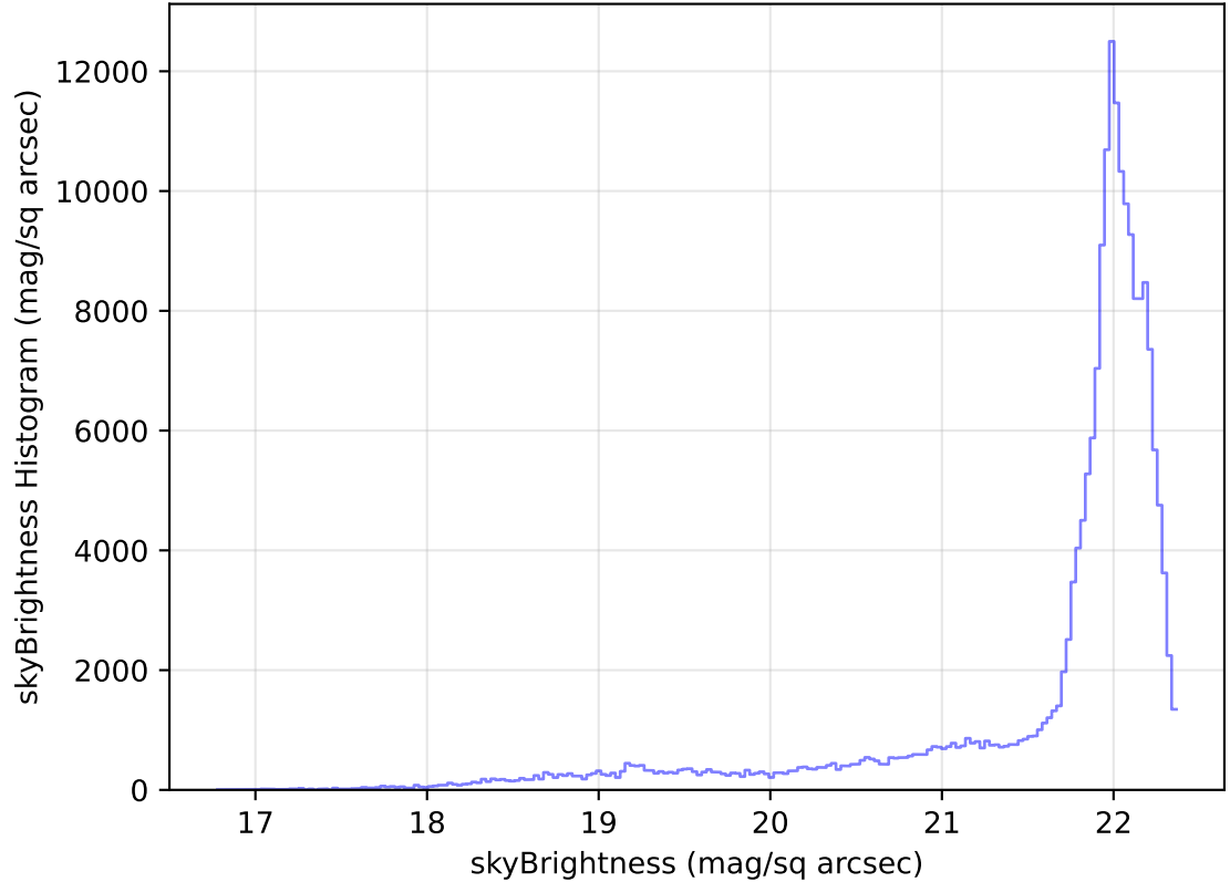
too_elab_heavy_r128_d2_ugrizy_v3.4_10yrs All sky g band: skyBrightness Histogram
