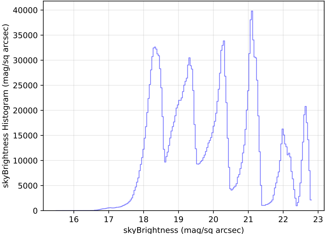
too_elab_heavy_r128_d2_ugrizy_v3.4_10yrs All sky all bands: skyBrightness Histogram
