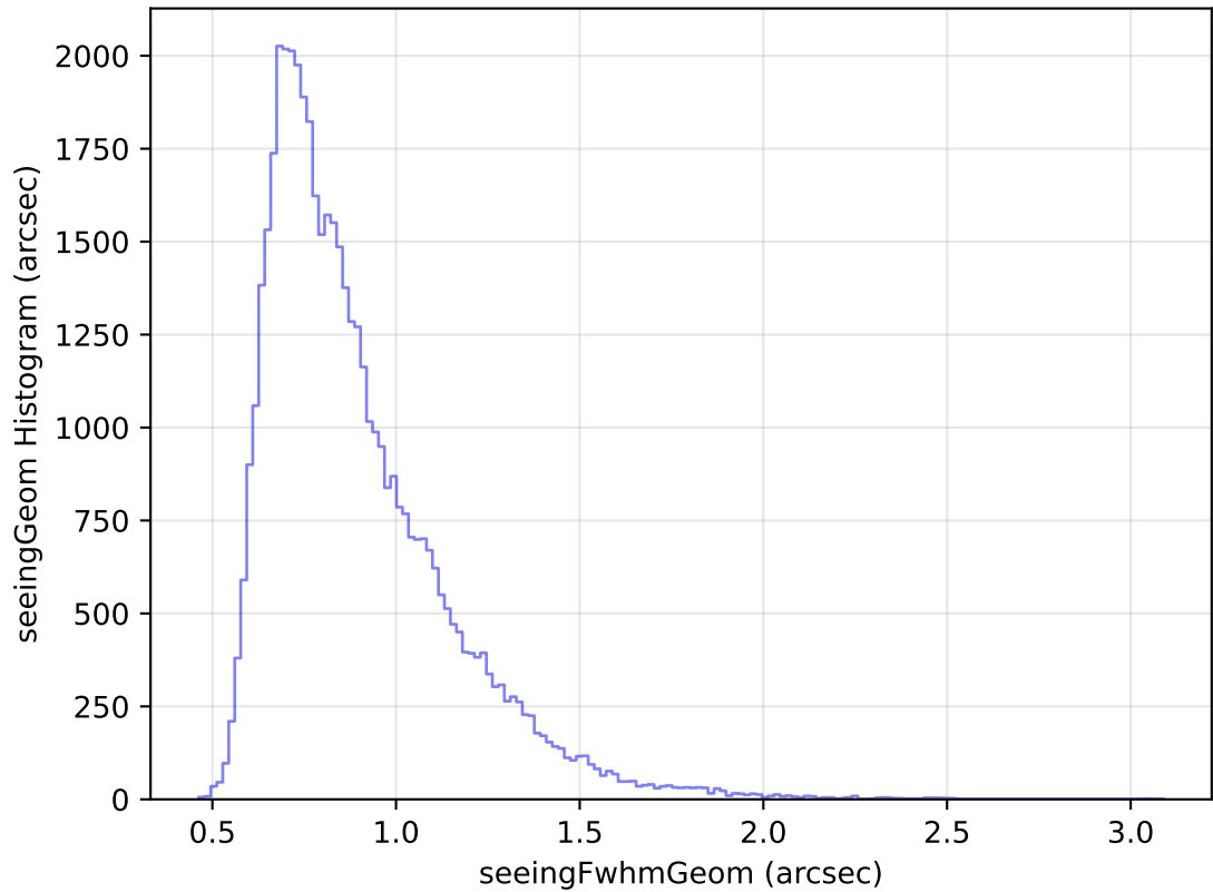
too_elab_heavy_r128_d2_ugrizy_v3.4_10yrs Yr 1 r band: seeingGeom Histogram
