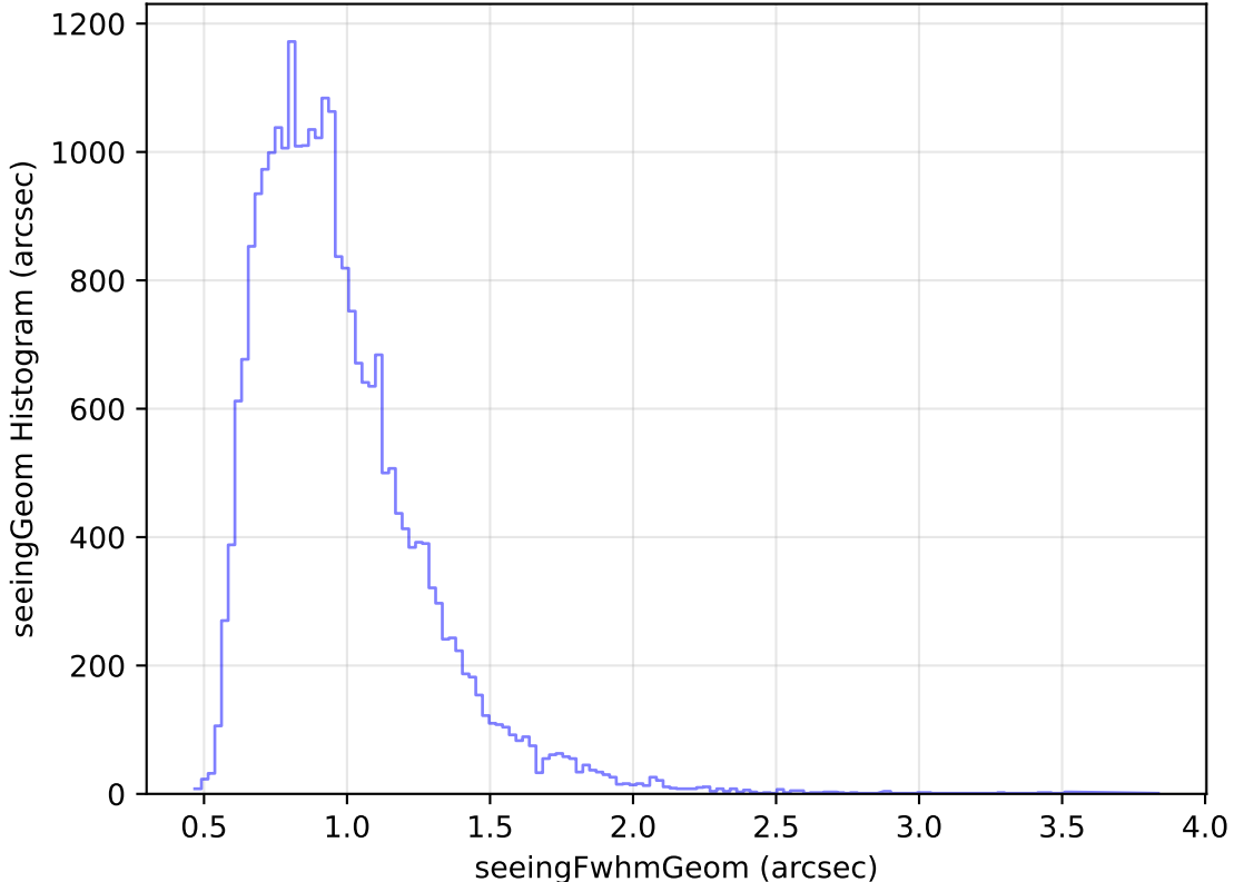
too_elab_heavy_r128_d2_ugrizy_v3.4_10yrs Yr 1 g band: seeingGeom Histogram
