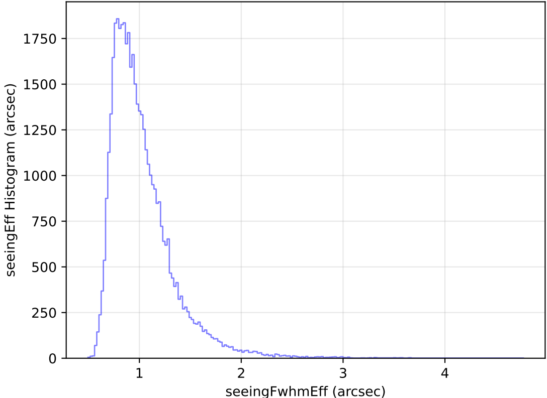
too_elab_heavy_r128_d2_ugrizy_v3.4_10yrs Yr 1 z band: seeingEff Histogram
