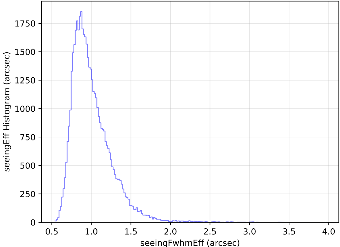
too_elab_heavy_r128_d2_ugrizy_v3.4_10yrs Yr 1 y band: seeingEff Histogram
