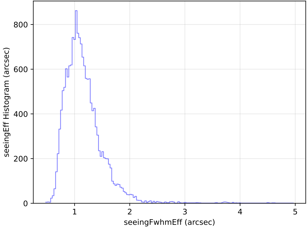
too_elab_heavy_r128_d2_ugrizy_v3.4_10yrs Yr 1 u band: seeingEff Histogram
