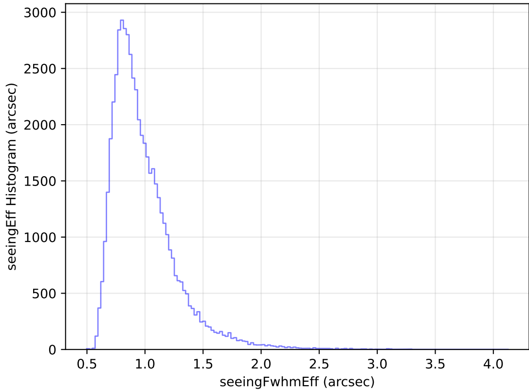
too_elab_heavy_r128_d2_ugrizy_v3.4_10yrs Yr 1 i band: seeingEff Histogram
