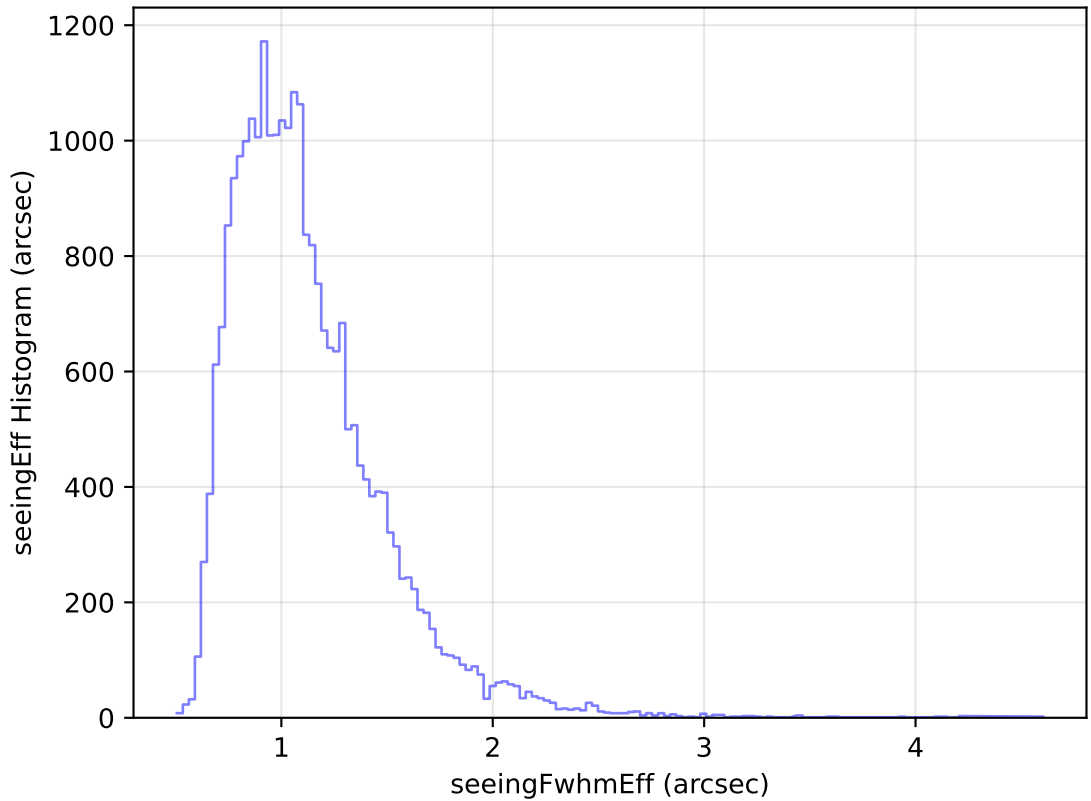
too_elab_heavy_r128_d2_ugrizy_v3.4_10yrs Yr 1 g band: seeingEff Histogram
