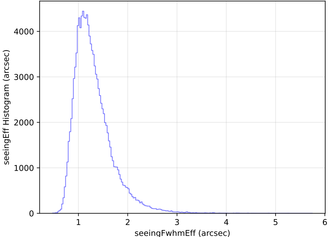
too_elab_heavy_r128_d2_ugrizy_v3.4_10yrs WFD u band: seeingEff Histogram
