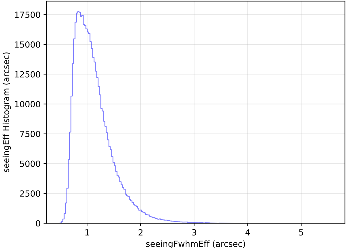
too_elab_heavy_r128_d2_ugrizy_v3.4_10yrs WFD r band: seeingEff Histogram
