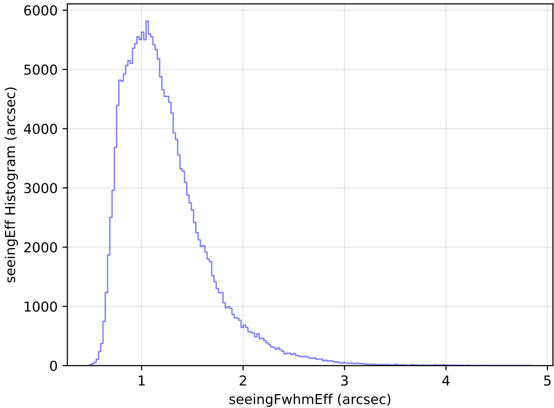
too_elab_heavy_r128_d2_ugrizy_v3.4_10yrs WFD g band: seeingEff Histogram
