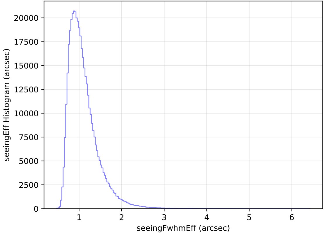
too_elab_heavy_r128_d2_ugrizy_v3.4_10yrs All sky z band: seeingEff Histogram
