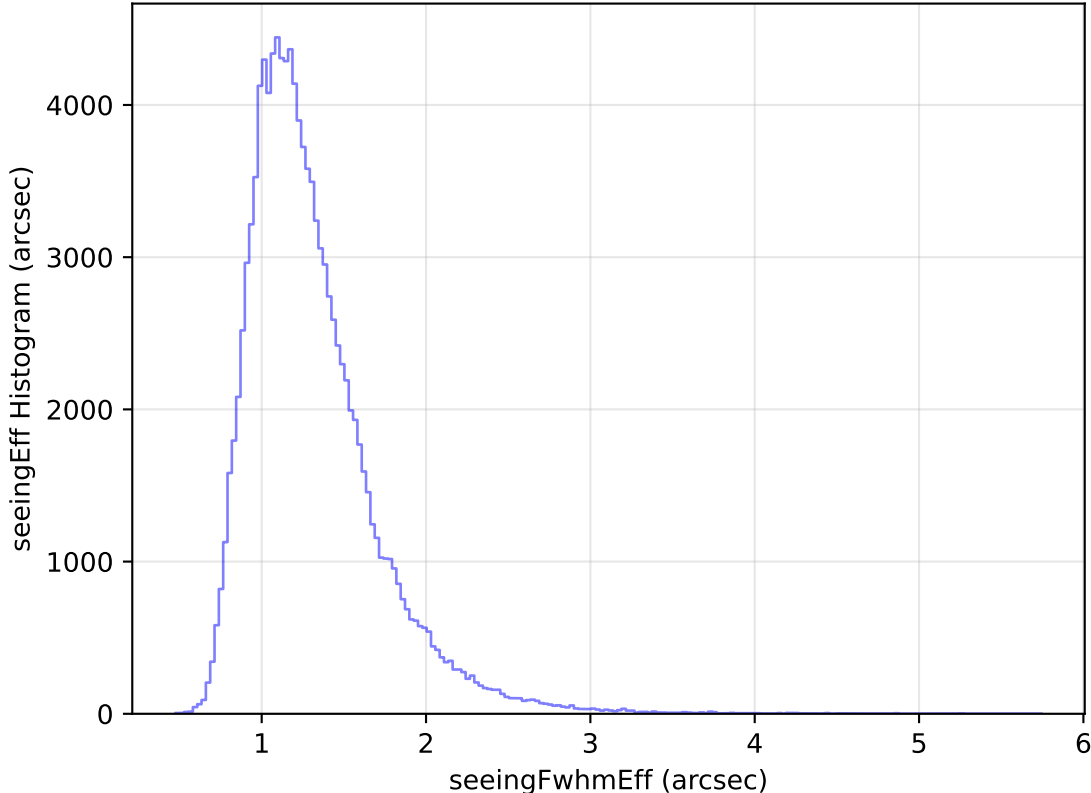
too_elab_heavy_r128_d2_ugrizy_v3.4_10yrs All sky u band: seeingEff Histogram
