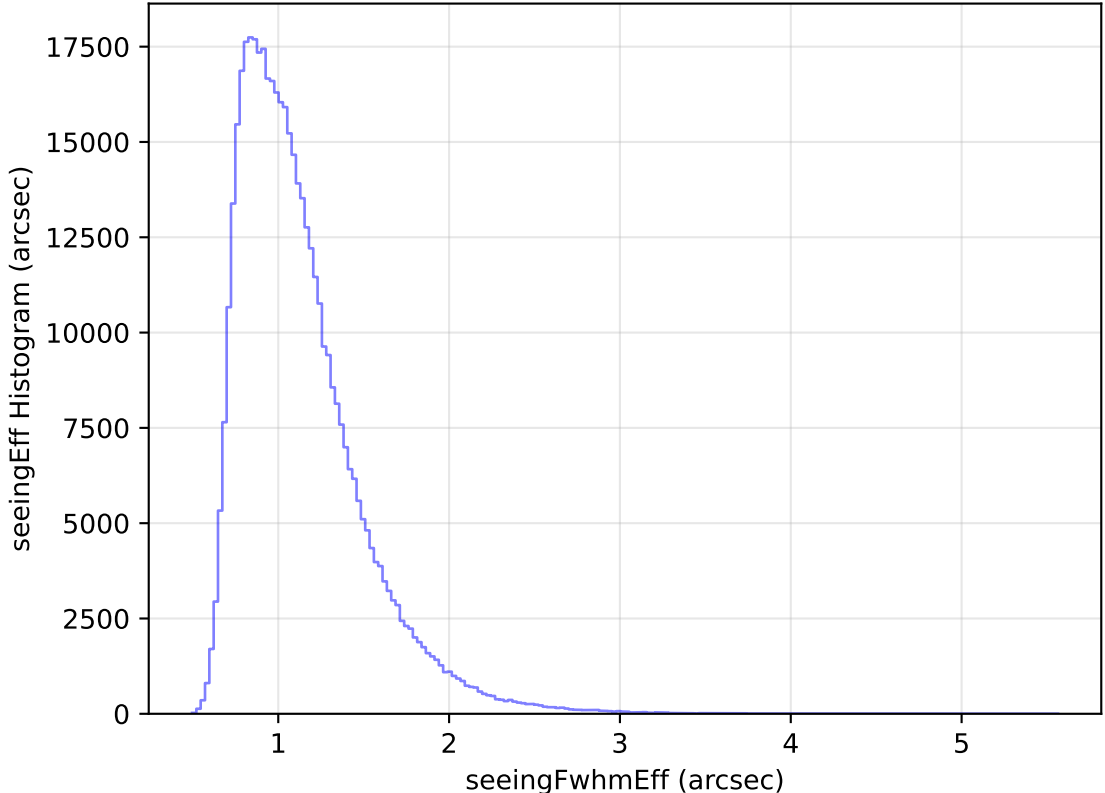
too_elab_heavy_r128_d2_ugrizy_v3.4_10yrs All sky r band: seeingEff Histogram
