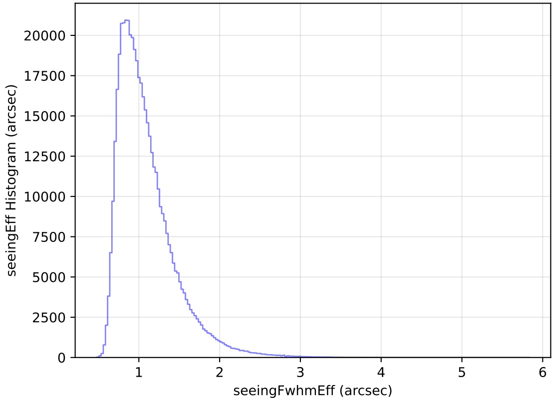
too_elab_heavy_r128_d2_ugrizy_v3.4_10yrs All sky i band: seeingEff Histogram
