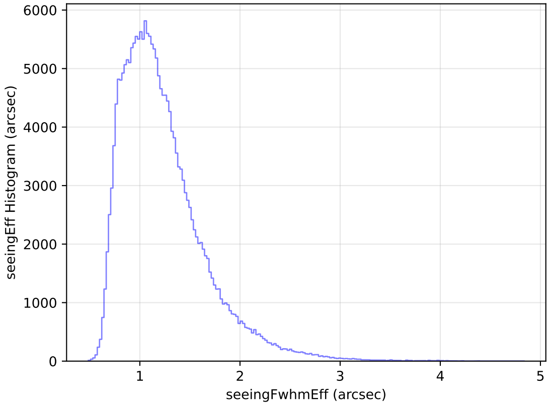
too_elab_heavy_r128_d2_ugrizy_v3.4_10yrs All sky g band: seeingEff Histogram
