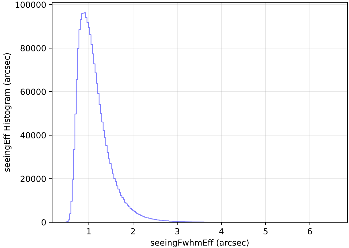
too_elab_heavy_r128_d2_ugrizy_v3.4_10yrs All sky all bands: seeingEff Histogram
