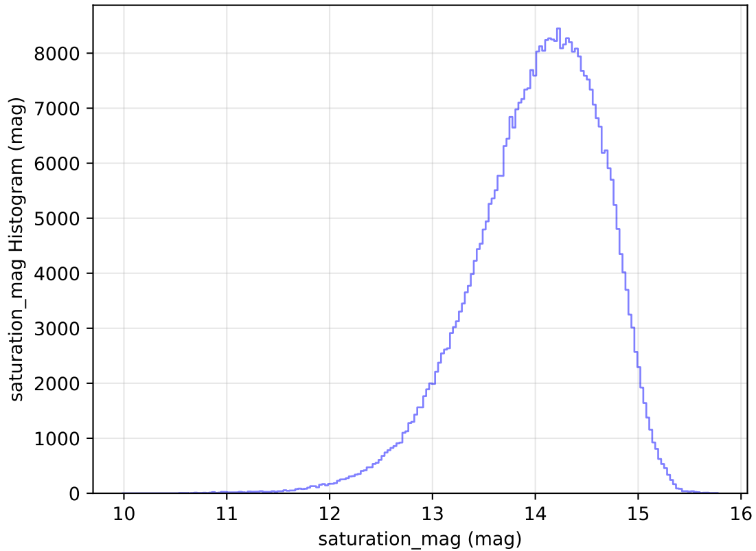
too_elab_heavy_r128_d2_ugrizy_v3.4_10yrs WFD z band: saturation_mag Histogram
